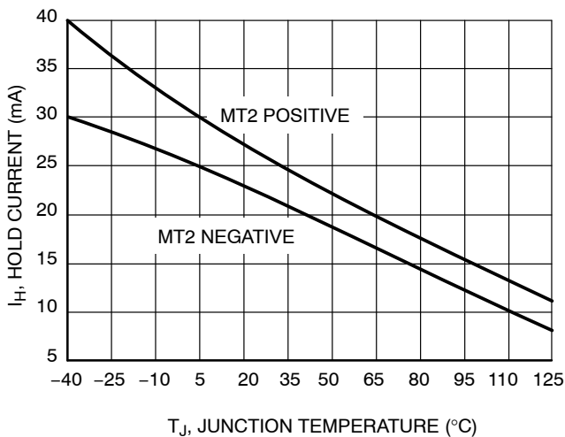
Figure 5. Typical Hold Current Variation
